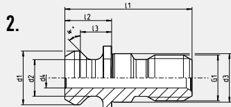
2. ISO 7388-3 Form UD con foro passante/Form UD with drill through (Norma precedente/previous norm ISO 7388-2 Form B)
