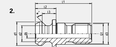
2. ISO 7388-3 Form UD con foro passante/Form UD with drill through (Norma precedente/previous norm ISO 7388-2 Form B)
